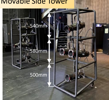
Movable Side Tower
